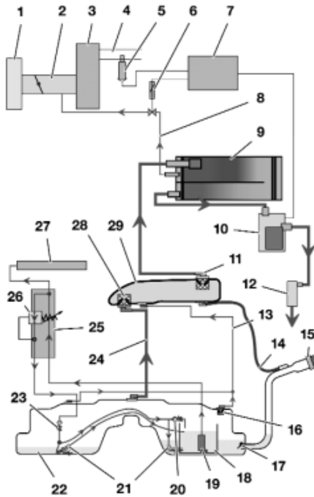
Fuel System
